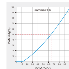
0/1-10V dimming
